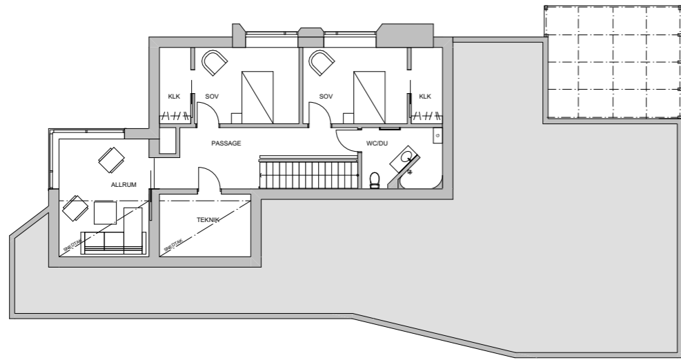
plan 2
