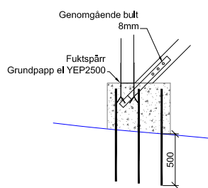
Grundplint/pelare/stag
